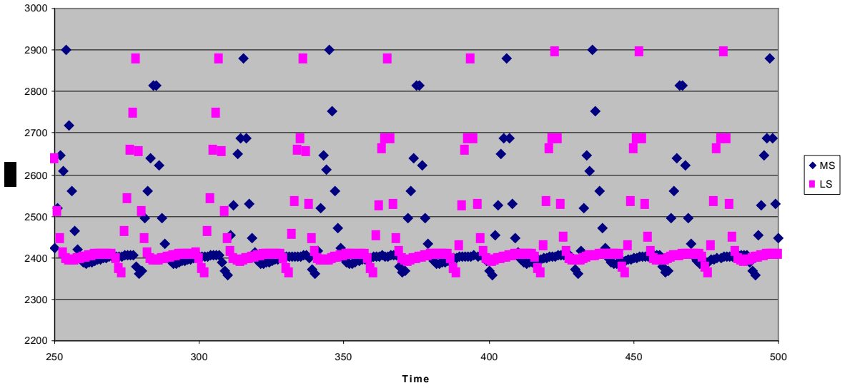
Figure 3 – Simultaneous ADCs readings during ERASE operations
